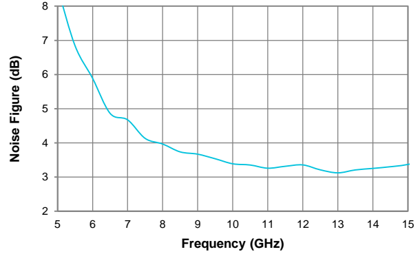
Noise Figure
